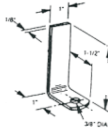
RC.7L 1" W. 3" H. 3/8" Hole
