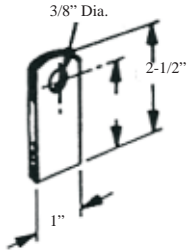
RC.2L 1" W. 2-1/2" H. 3/8" Hole
