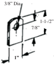
RC.3 1" X 1-1/2"H. 3/8" Hole 8 Ga
