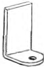
RC.8L 1-1/2" W. 3" H. 3/8" Hole
