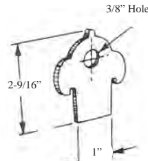
RC1.S 1" Base 2-9/16" H.
